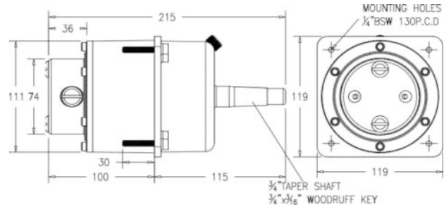
OPTIONAL Model 101 & 102 Mid-mount helm unit
