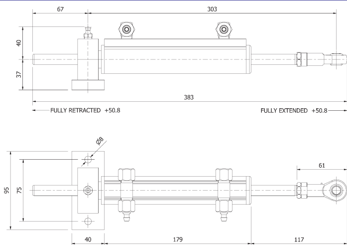
Model 512JET Cylinder dimensions
