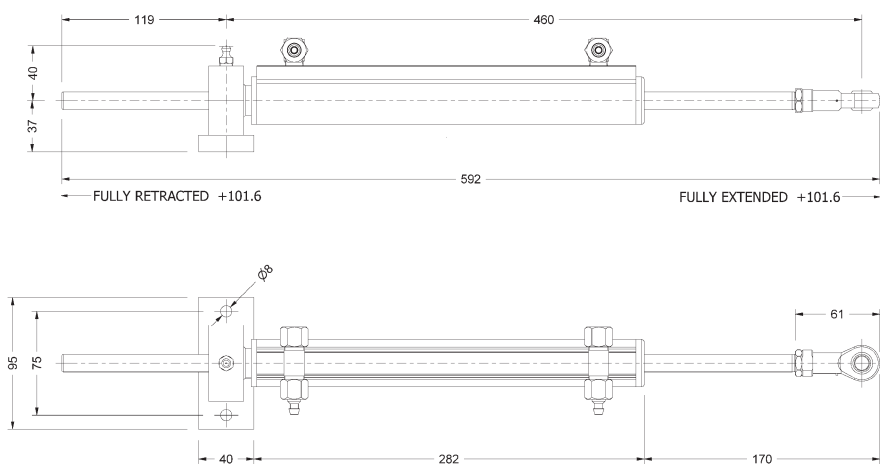
Model 512 Cylinder dimensions
