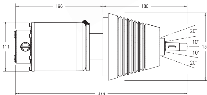
Fully tilting helm design Model 101 - Tilt or 102 - Tilt
