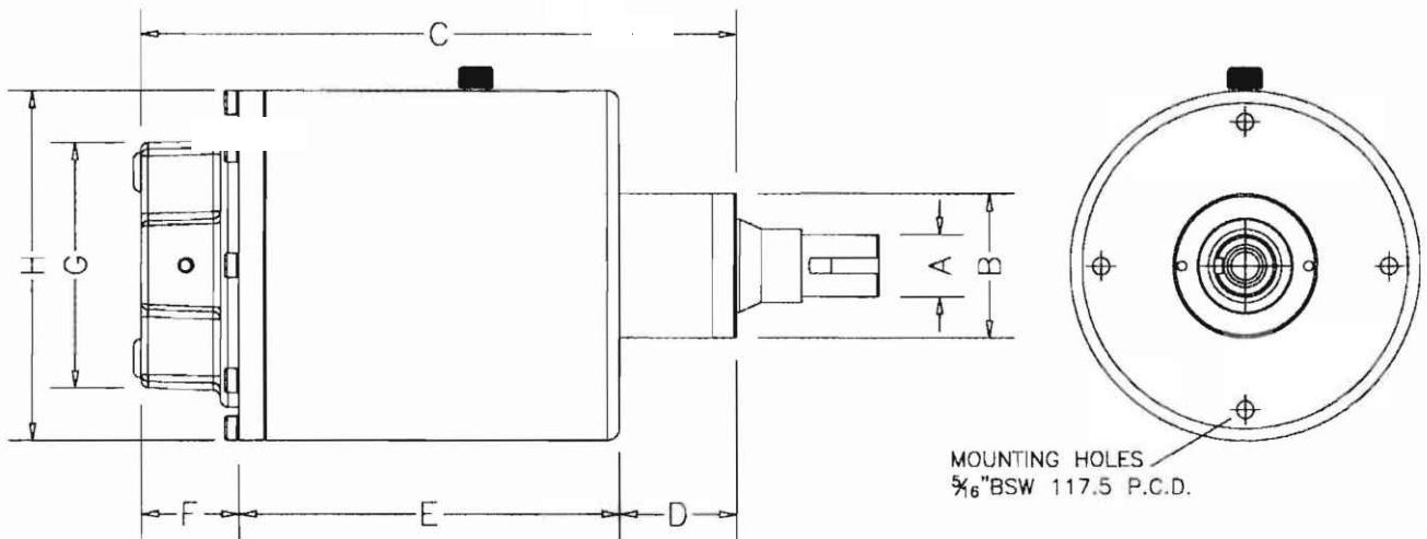
Model 103,104,105,106 &107 HELM PUMP DIMENSIONS
