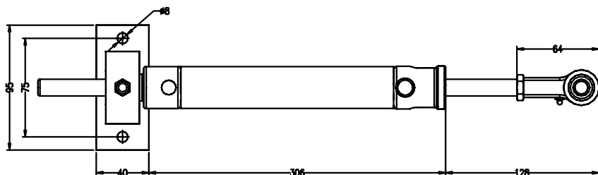
Model 212 Cylinder dimensions
